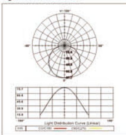
Light Distribution Curve
