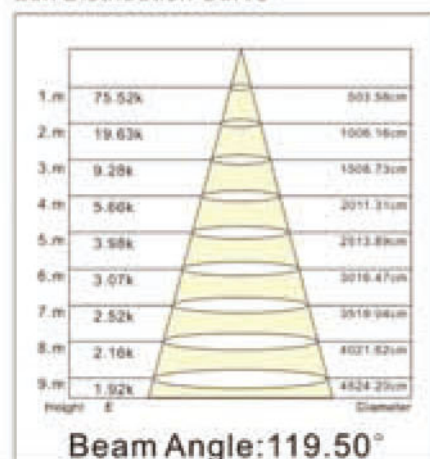
Lux Distribution Curve
